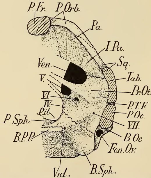
FIG. 14.— Cynariops robustus . Type. Lateral view of the left side of the brain-case. \times \frac{1}{4} .
